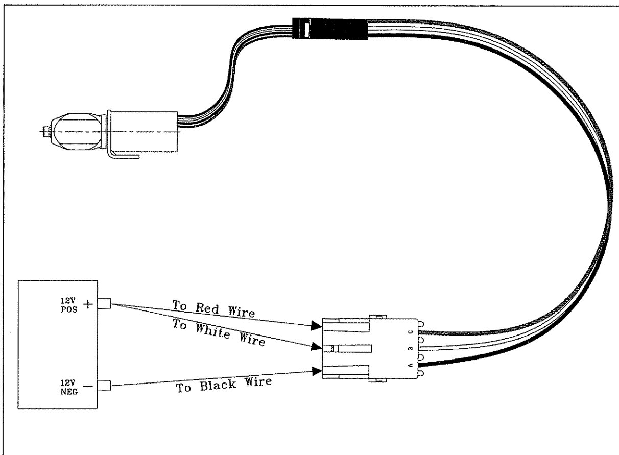
Diagram "C" Three-Wire Solenoid Test
